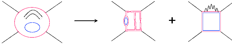
Figure 2. A world-sheet with one handle and two boundaries that contributes to the single-trace term at the same order as the four-boundary amplitude of figure 1. The figure illustrates examples of field theory diagrams that arise from the short-handle and long-handle boundaries of moduli space in the low energy limit.
