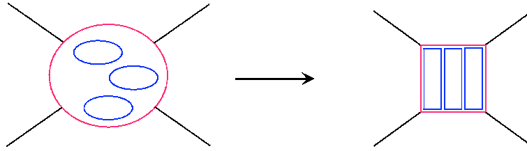
Figure 1. Three-loop contribution to the single-trace term in four-gluon scattering and its connection to the \text{tr}F^4 term in Yang-Mills theory in the low energy limit.
